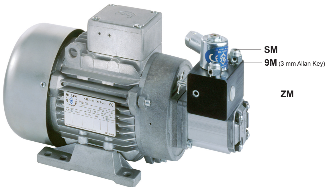
Micro Drive Unit (1,0 to 24 lpm) (0,3 to 7,5 gpm)
